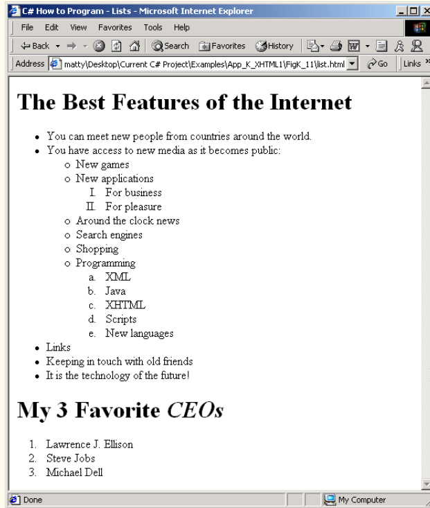
Fig. K.10 Nested and ordered lists in XHTML. (Part 3 of 3.)
