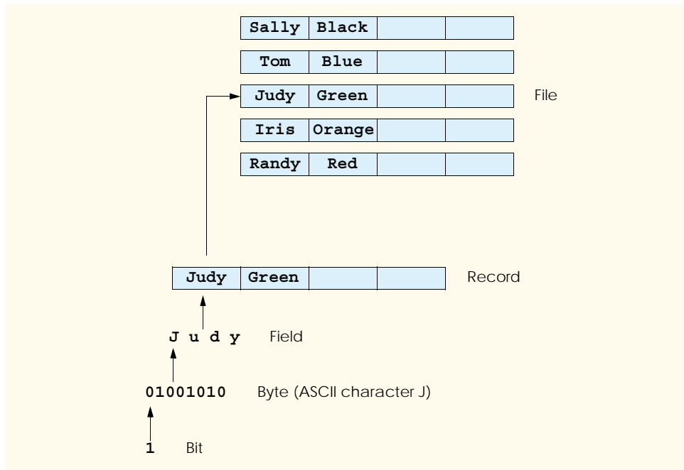
Fig. 17.1 Data hierarchy.
