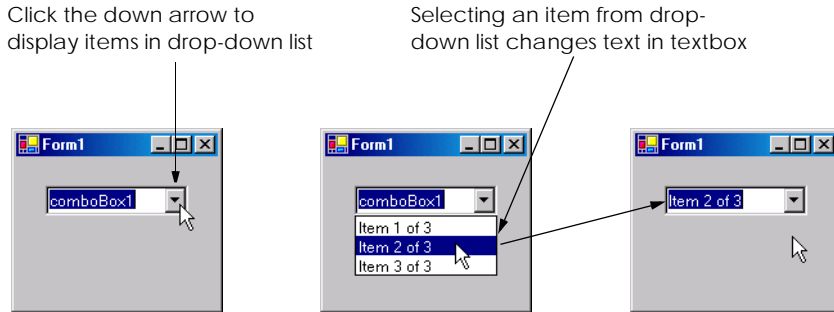
Fig. 13.14 ComboBox demonstration.
