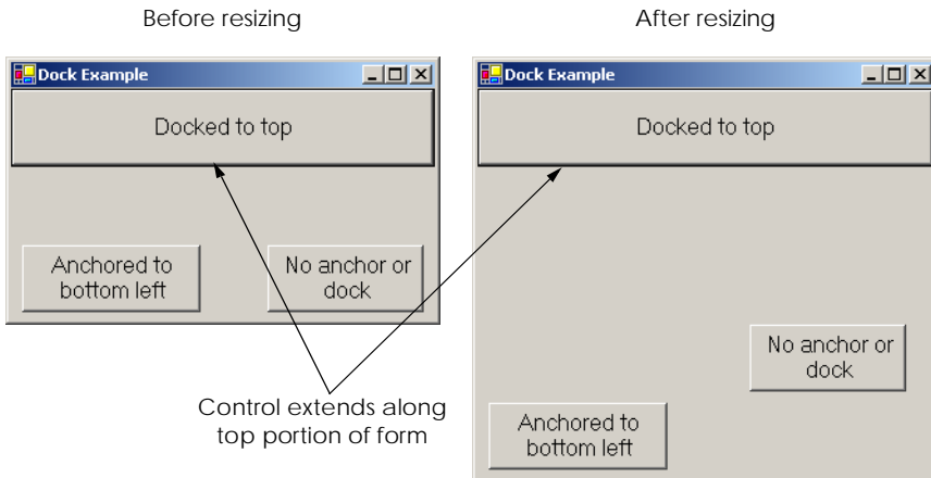
Fig. 12.13 Docking demonstration.
