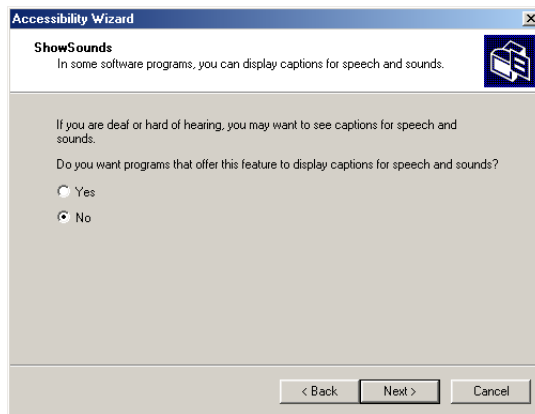
Fig. 24.29 ShowSounds dialog.
