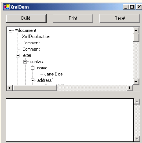
Fig. 18.8 DOM structure of an XML document illustrated by a class. (Part 5 of 6.)
