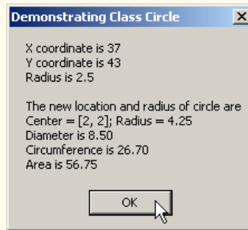
Fig. 9.7 CircleTest demonstrates class Circle functionality. (Part 2 of 2.)
