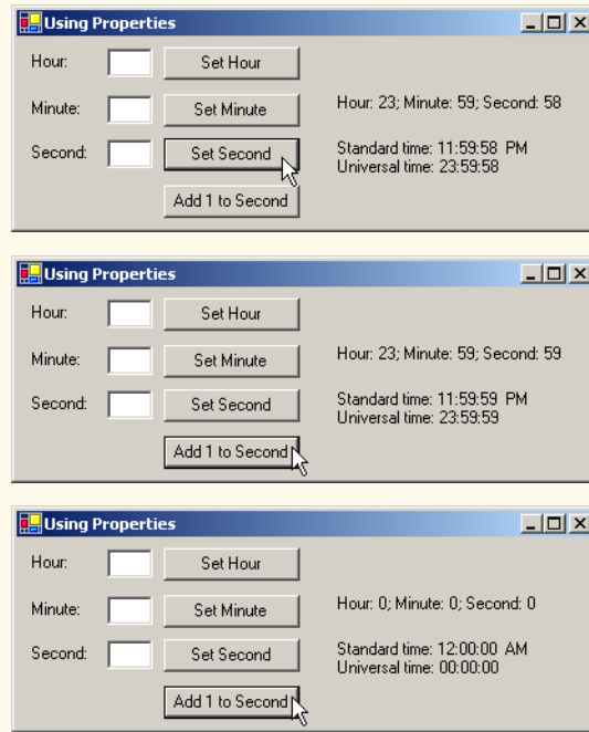
Fig. 8.7 Properties demonstration for class Time3 . (Part 5 of 5.)
