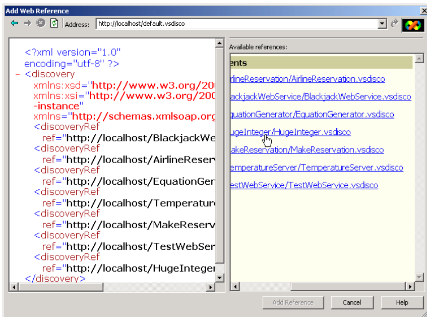
Fig. 21.10 Web services located on localhost.
