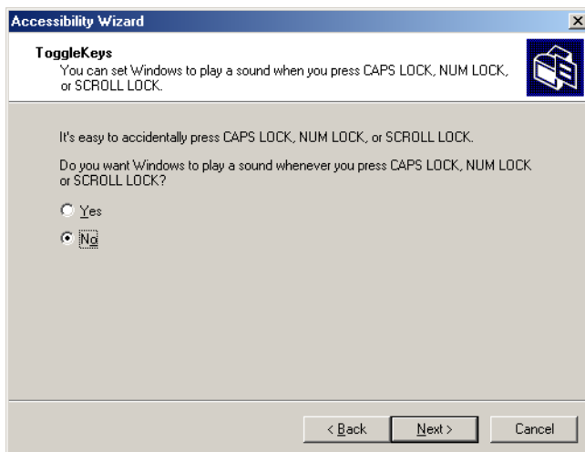
Fig. 24.32 ToggleKeys window.
