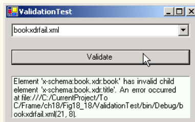
Fig. 18.22 XML file that does not conform to the Schema in Fig. 18.17. (Part 2 of 2.)
