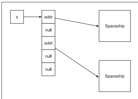
Figure 4.5 An array of references, where some are valid and others are null.
