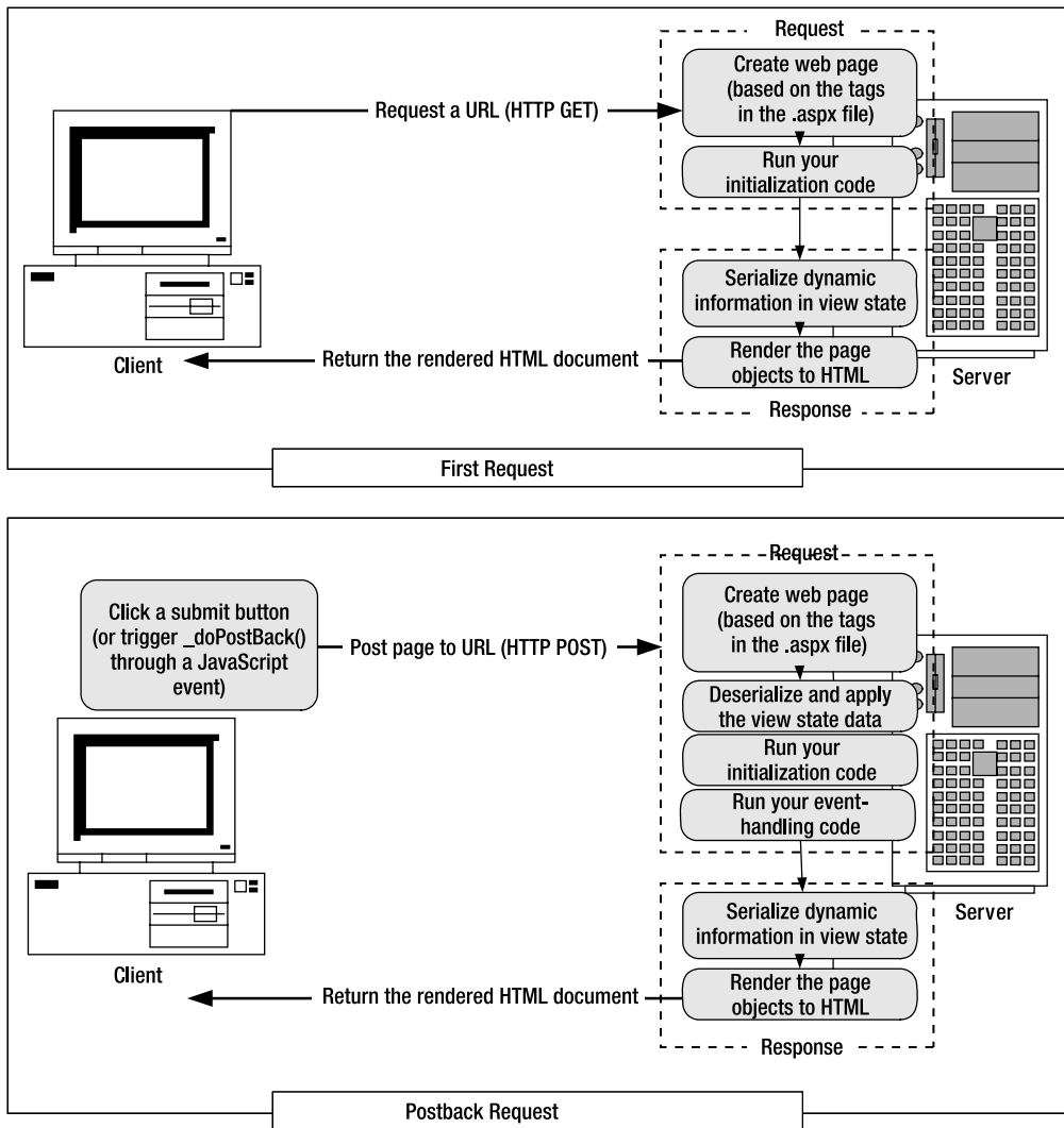
Figure 3-2. ASP.NET page requests
