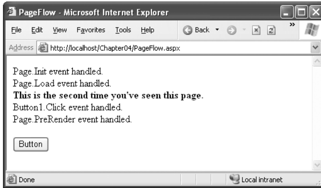
Figure 3-5. ASPNET order of operations
