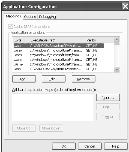
Figure 23-7. Application mappings
