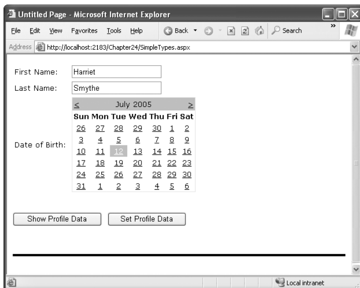
Figure 24-2. Testing profiles
