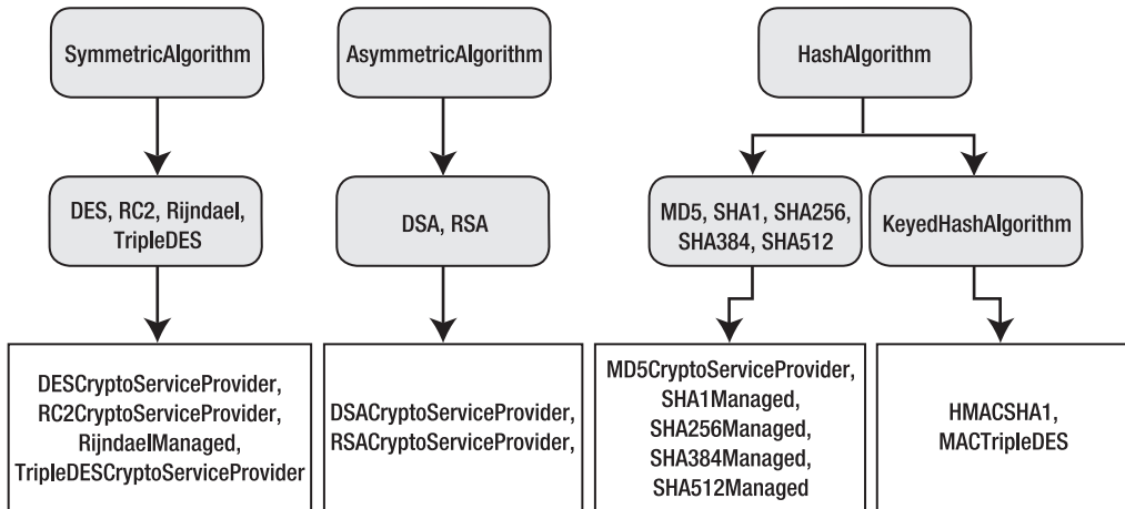
Figure 25-2. The cryptographic class hierarchy
