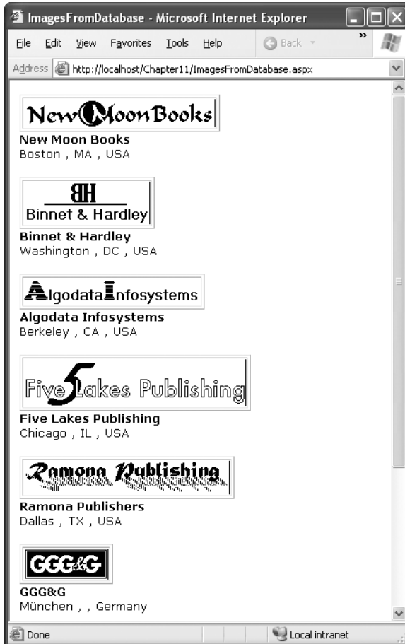
Figure 10-23. Displaying database images in ASP.NET web page
